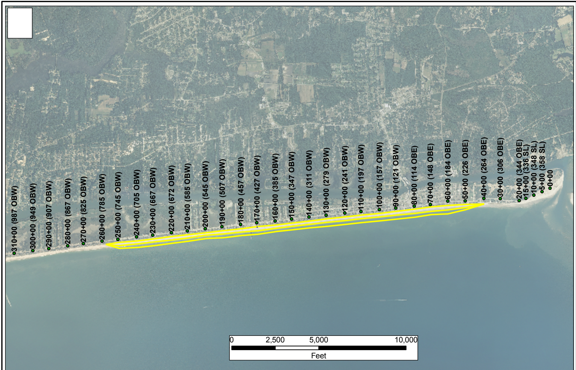
FIGURE 1 Holden Beach Central Reach Fill Template
